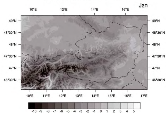
Inca Mean Monthly Temperature
