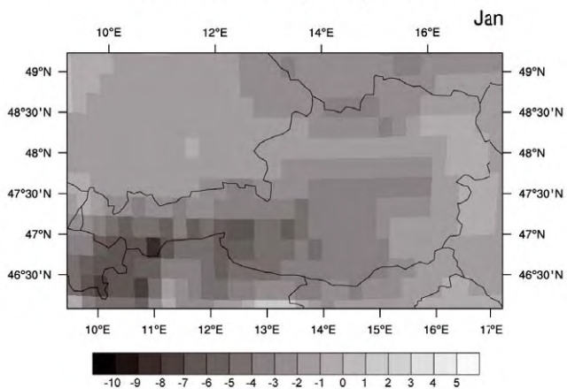
Eobs Mean Monthly Temperature
